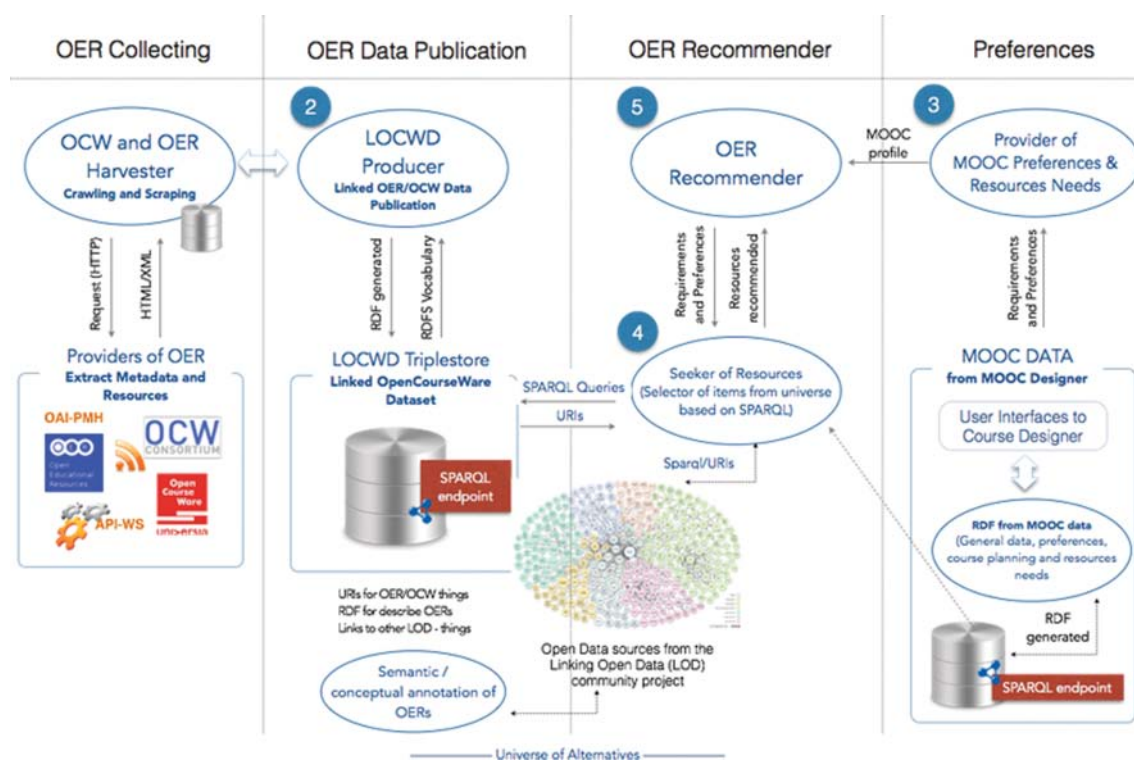
Figure 1: Architecture for Seeker of OER from Linked OpenCourseWare and OER Data (LOCWD) Triplestore
