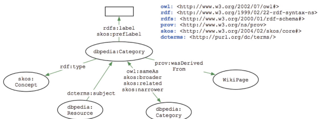
Figure 2: Key resources used for OER annotation and enrichment from DBPedia
