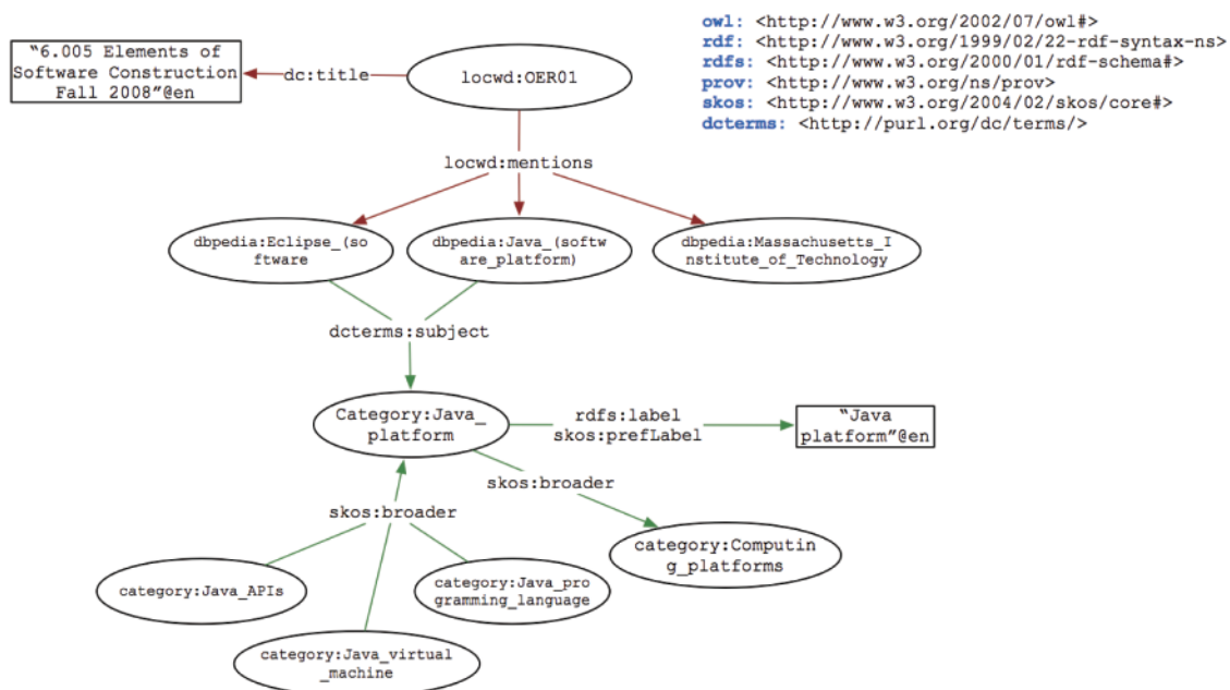
Figure 3: An example of annotation of OER from DBPedia. The annotation process not only provides access to a large amount of structured data sources but also enables machines and software agents to automatically analyze this semantic knowledge
